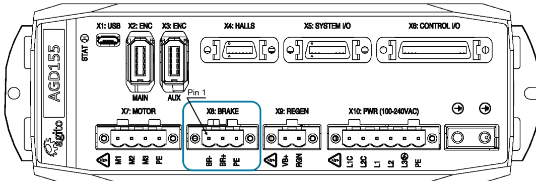
Figure 12. Brake Connector
