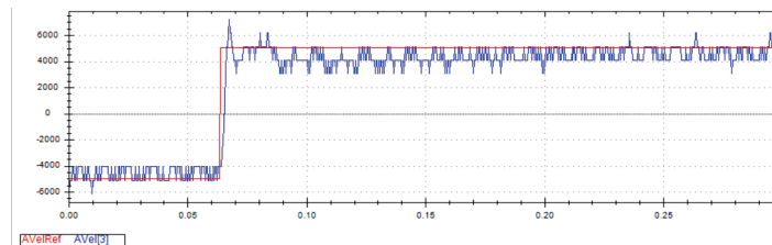
Figure 54. Typical Velocity Loop Performance
