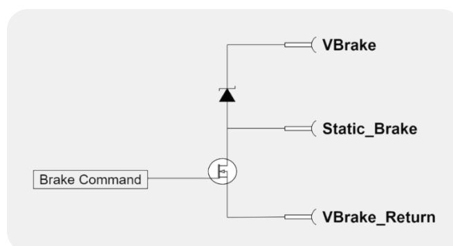
Figure 13. Electrical Interfaces – Static Brakes
