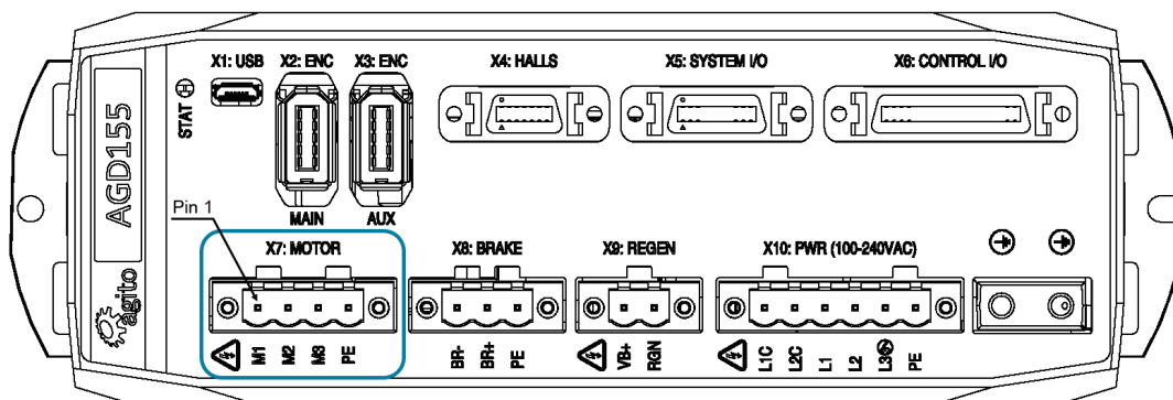
Figure 11. Motor Connector
