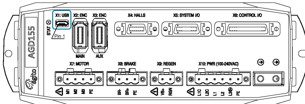
Figure 19: USB Connector
