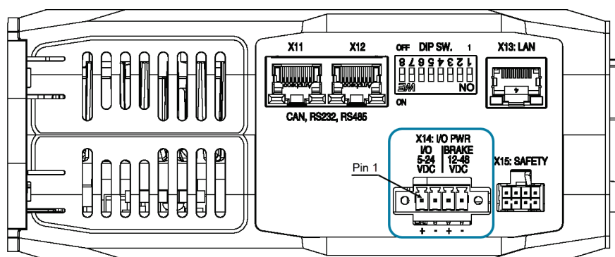
Figure 8. I/O and Brake Power Connector
