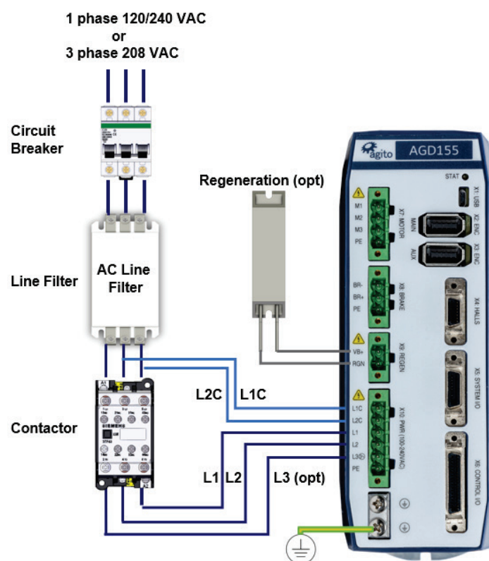
Figure 5. Power supply wiring
