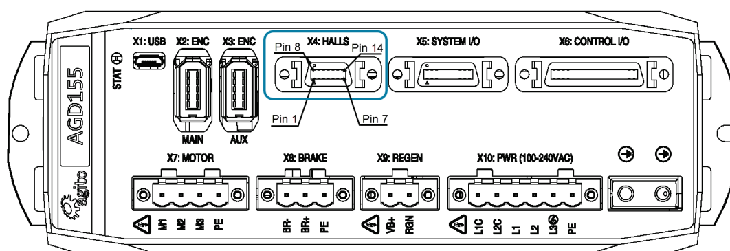
Figure 22. Hall Sensors Connector
