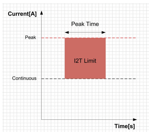
Figure 38. I^2T
