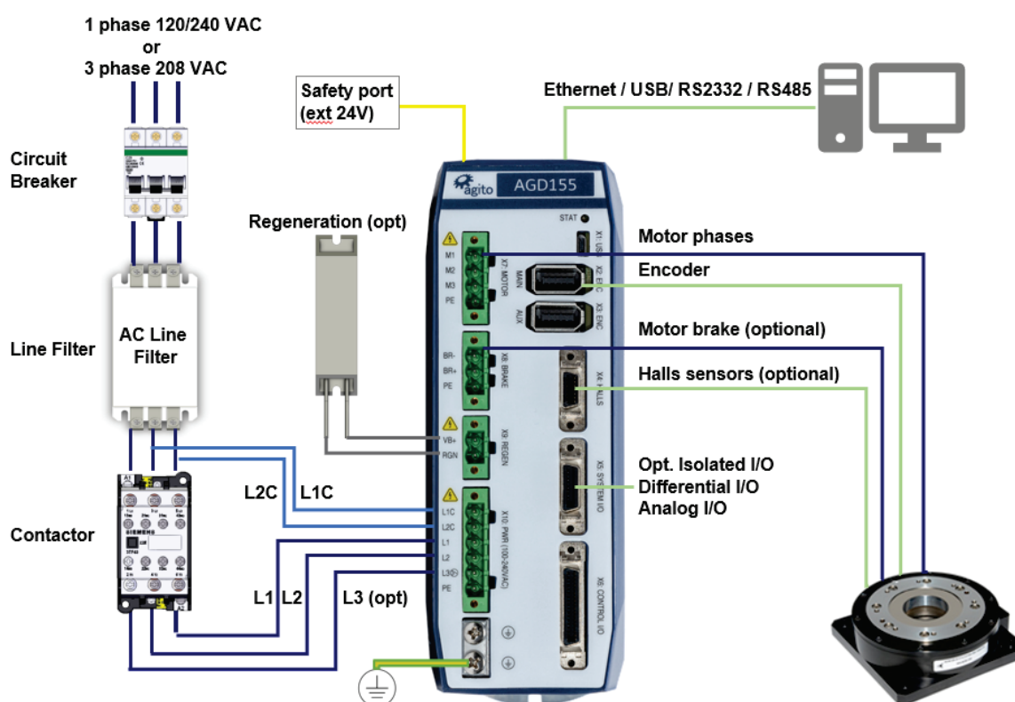
Figure 2. System connections and wiring
