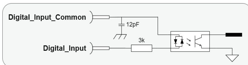
Figure 25. Electrical Interfaces – Digital Input 1 to 3, 5 to 9, and 13 to 16 (3 isolated groups)
