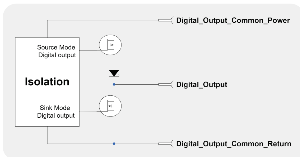
Figure 27. Electrical Interfaces – Digital Output 1 to 2, and 3 to 6
