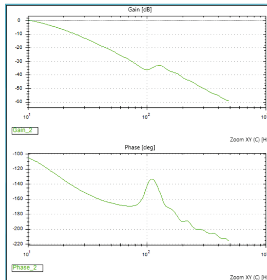
Figure 48. Typical Plant Transfer Function
