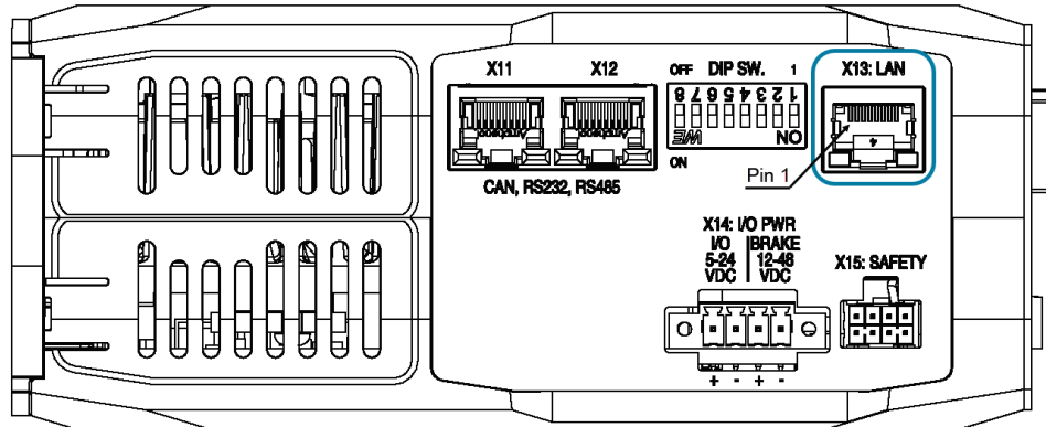
Figure 17: Ethernet Connector
