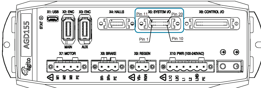
Figure 23. System I/O Connector
