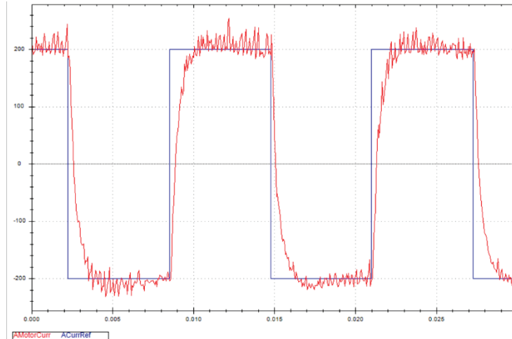
Figure 46 Typical Current Loop Performance
