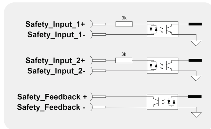
Figure 10. Electrical Interfaces – Safety Connector
