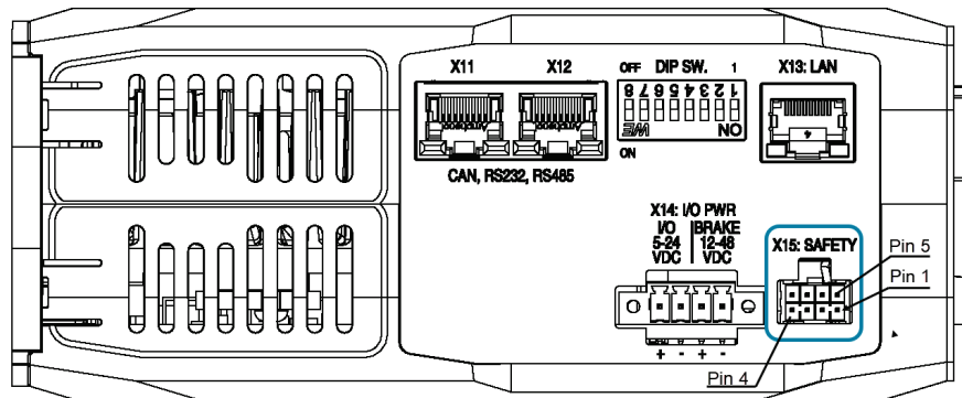
Figure 9. Safety Connector
