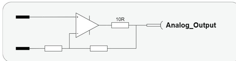
Figure 31. Electrical Interfaces – Analog Output 1 to 2
