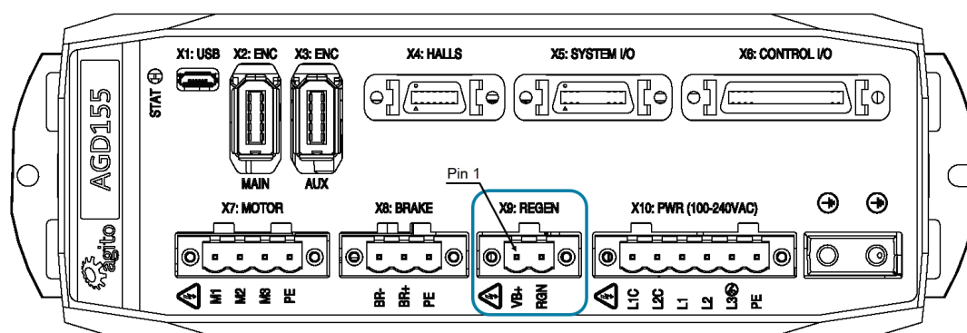
Figure 14. Regeneration Connector
