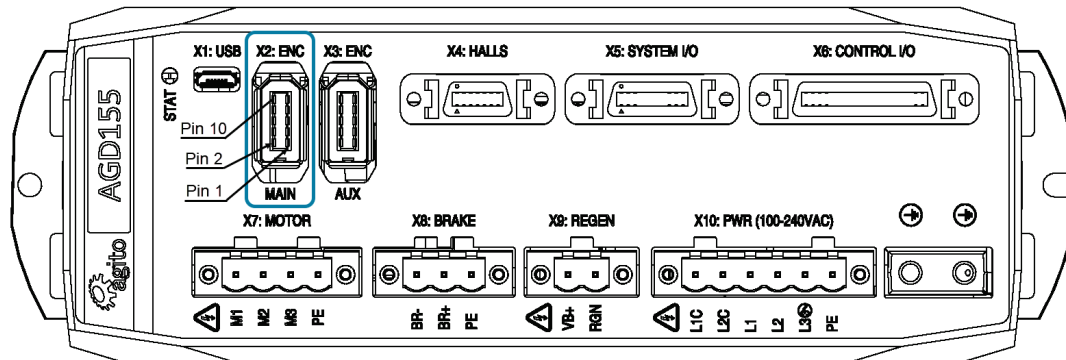
Figure 20. Main Encoder Connector
