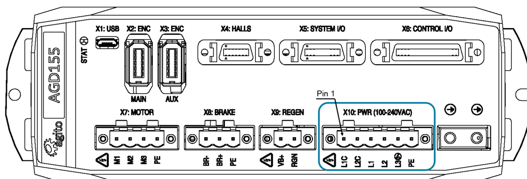
Figure 16. Power Connector
