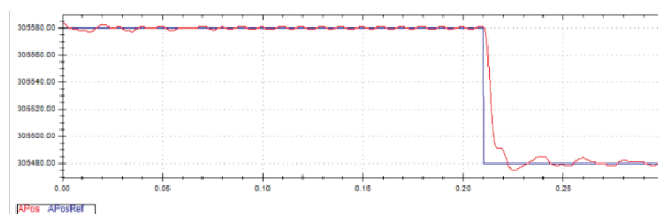
Figure 56. Typical Position Loop performance
