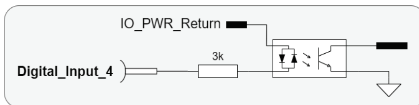
Figure 26. Electrical Interfaces – Digital Input 4
