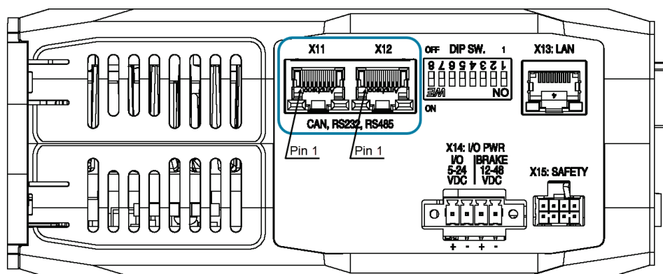
Figure 18: Serial Communication Connectors
