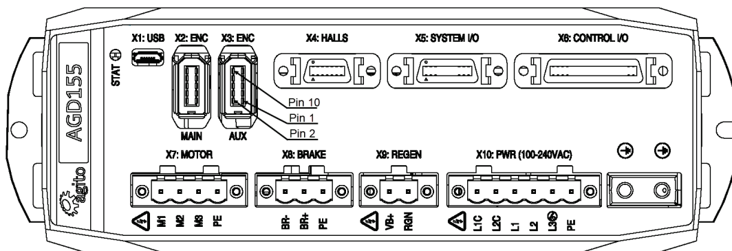
Figure 21 Aux Encoder Connector
