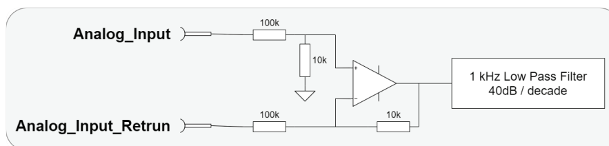
Figure 30. Electrical Interfaces – Analog Input 1 to 2
