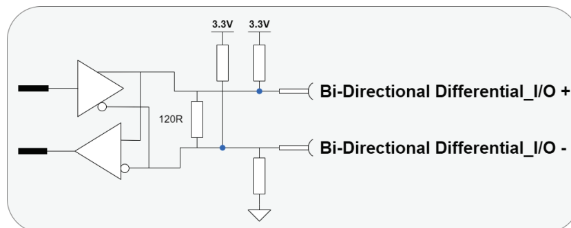
Figure 29. Electrical Interfaces – Bi-Directional Differential I/O
