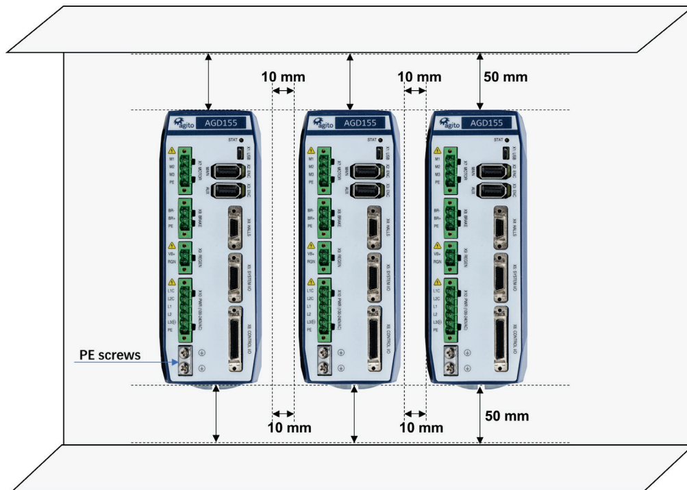
Figure 4. Mounting multiple amplifiers within cabinet
