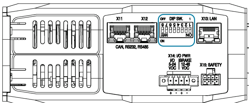
Figure 15 DIP Switches
